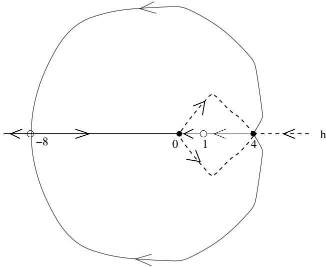
Fig. 2. The preimage by H of the real line
