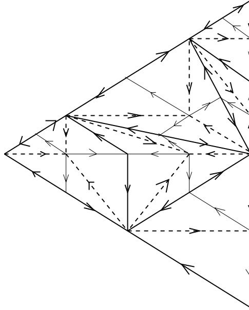
Fig. 6. The combinatorics of the triangulation \mathcal{T}_3
