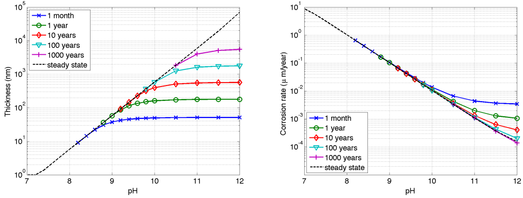
Figure 6.2: Thickness of the oxide layer (left) and corrosion rate (right) depending on pH value.
