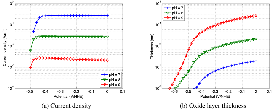
Figure 6.1: Current density and oxide layer thickness after reaching pseudo steady state vs. applied potential, for different pH values in claystones. Parameter values are given in Table 6.1.
