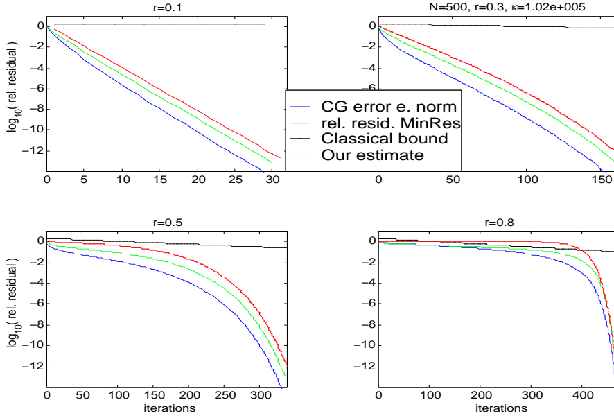
FIG. 3. The one dimensional Poisson problem discretized on a uniform grid ( N = 500 ) for f(x) = \sum_{j=1}^N r^j \sin(j\pi x) , r = 0.1, 0.3, 0.5, 0.8 . We find the CG (relative) error curve (energy norm) in blue, the classical bound (1.1) in black, and our new asymptotic bound in red. For comparison we give the MINRES relative residual curve in green.
