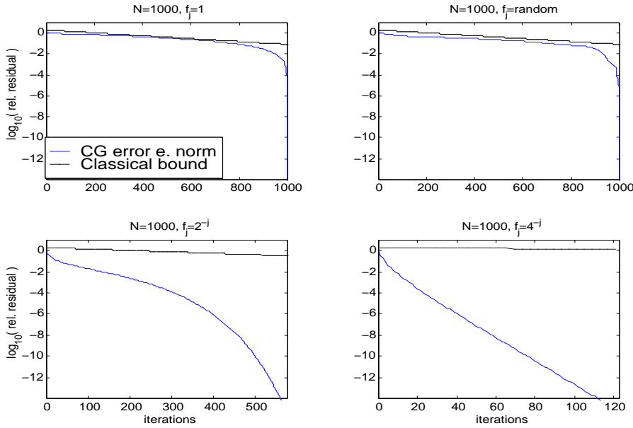
FIG. 1. The CG relative error curve (energy norm, blue) for the one dimensional Poisson problem discretized on a uniform grid ( N = 1000 , x_{0,N} = 0 ) for four choices of f(x) = \sum_{j=1}^N f_j \sin(j\pi x) : there is hardly any superlinear convergence for the upper two examples ( f_j = 1 , f_j random) and one has to reach approximately the dimension of the system in order to achieve full precision. In contrast, for the lower two examples ( f_j = 2^{-j} , f_j = 4^{-j} ) we observe superlinear convergence. For the sake of completeness, we have also drawn in black the error bound (1.1) for the four examples. This bound is only significant for the first two examples.
