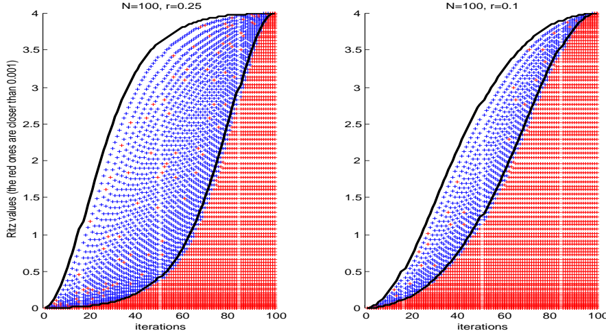
FIG. 2. Convergence of Ritz values for our model problem with N = 100 , x_{0,N} = 0 , and f(x) = \sum_{j=1}^N r^j \sin(j\pi x) , r \in \{1/4, 1/10\} . The two black curves indicate the graphs of \alpha, \beta . We draw in the n th column, 1 \leq n \leq N , the position of the n th Ritz values (red or blue) within the interval [0, 4] . A red cross is used if the Ritz value is closer than 0.001 to some eigenvalue of A_N . Notice that nearly all Ritz values are red in the range [0, \alpha(t)] , t = n/N , that there are no Ritz values in [\beta(t), 4] , and that in the range [\alpha(t), \beta(t)] hardly any Ritz value converged (up to some exceptions by “accident”).
