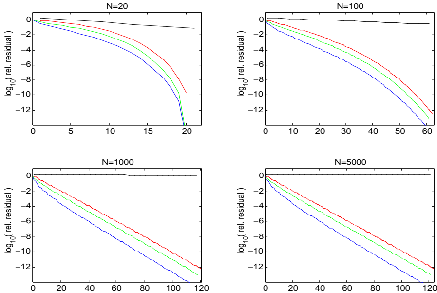
FIG. 4. The one dimensional Poisson problem discretized on a uniform grid for f(x) = \sin(\pi x)/[r^2 + 1 - 2r \cos(\pi x)] , r = 1/4 , and N = 20, 100, 1000, 5000 . We find the CG (relative) error curve (energy norm) in blue, the MINRES relative residual curve in green, the classical bound (1.1) in black, and our new asymptotic bound in red.
