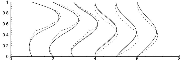
Fig. 3. Averaged transversal horizontal velocity profiles for Re = 500 . Dashed : Level 1, Dotted : Level 2, Plain : Level 3.
