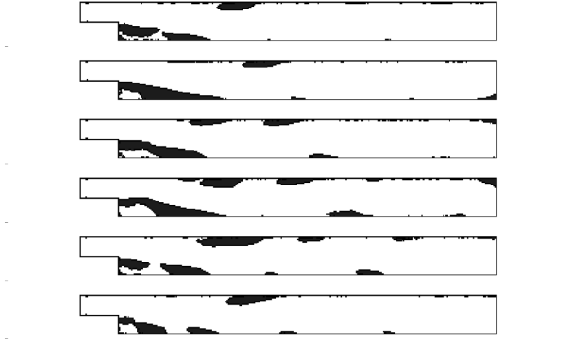
Fig. 13. Horizontal velocity u < 0 from t = 592.5 to t = 600.0 , with \Delta t = 1.5 , closed-loop controlled (non-intrusive) regime.
