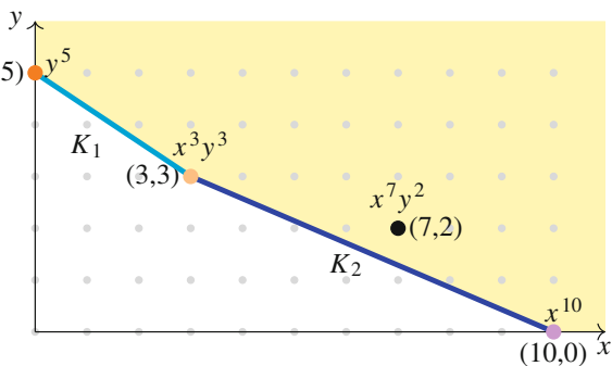
Fig. 1.4 The Newton polygon of the series f(x, y) = (y^2 - 2x^3)(y^3 - x^7)
