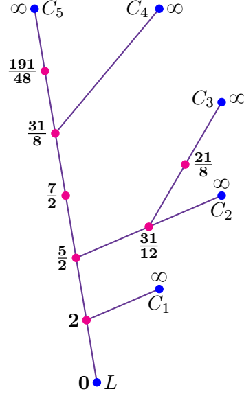
FIGURE 6. The values of the contact complexity \mathbf{c}_L at the marked points of the tree of Example 3.13
