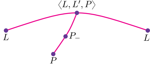
FIGURE 21. The case P \in \mathbb{P}(\mathcal{V}) \setminus [L, L']
