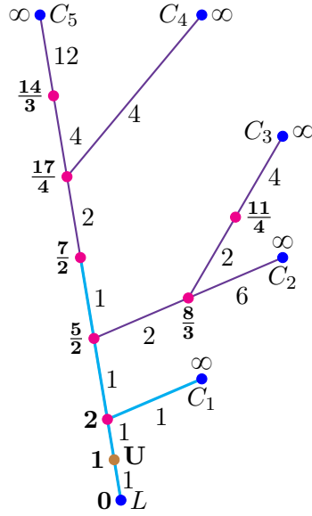
FIGURE 7. The unit subtree (in heavier lines) and the unit point of the Eggers-Wall tree (labelled by U )
