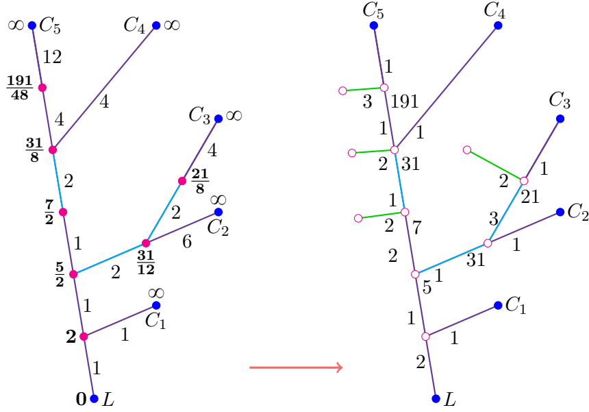
FIGURE 13. The splice diagram associated to our recurrent example
