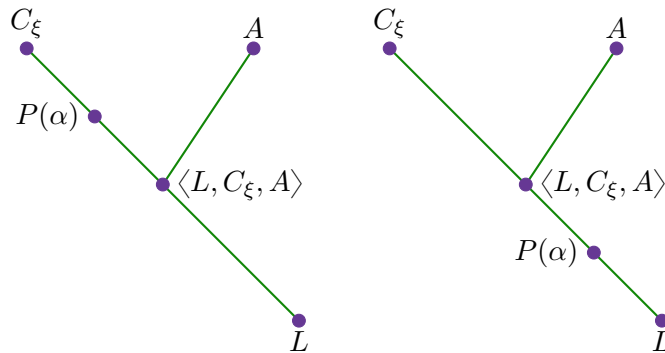
FIGURE 15. One has to compare P(\alpha) and \langle L, C_\xi, A \rangle
