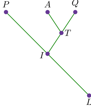
FIGURE 17. The case when P and Q are incomparable
