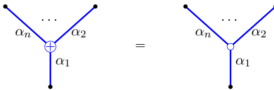
FIGURE 10. The splice diagram of the oriented homology sphere \Sigma(\alpha_1, \dots, \alpha_n) .
