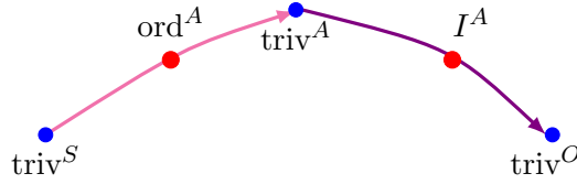
FIGURE 14. The orbits of \text{ord}^A and of I^A
