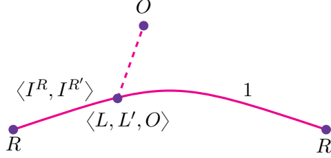
FIGURE 18. Some values of \mathbf{m}_{R'}
