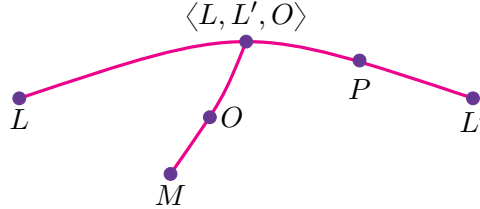
FIGURE 19. The case P \in [L', \langle L, L', O \rangle]
