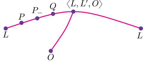
FIGURE 20. The case P \in (\langle L, L', O \rangle, L]
