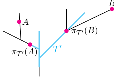
FIGURE 3. Attaching points on a subtree
