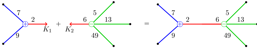
FIGURE 11. Splicing two star-shaped diagrams along the knots K_1 and K_2 .
