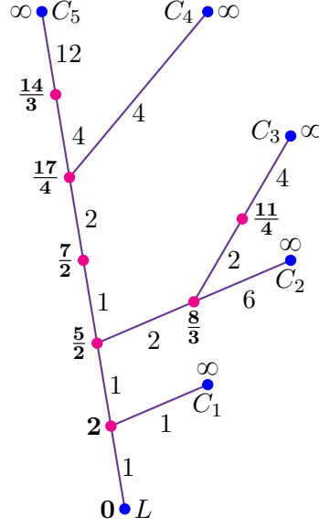
FIGURE 5. The Eggers-Wall tree of Example 3.13
