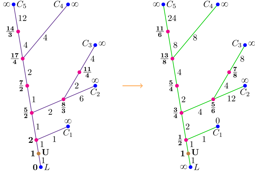
FIGURE 9. The Eggers-Wall trees \Theta_L(C) of Example 4.10 on the left, compared with \Theta_{C_1}(C) on the right.
