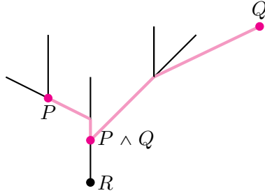
FIGURE 1. The infimum of two elements in a rooted tree
