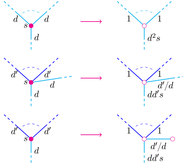
FIGURE 12. From the Eggers-Wall tree to the splice diagram
