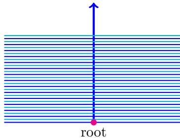
FIGURE 2. An example of \mathbb{R} -tree
