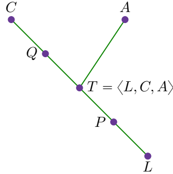
FIGURE 16. The case when P and Q are comparable
