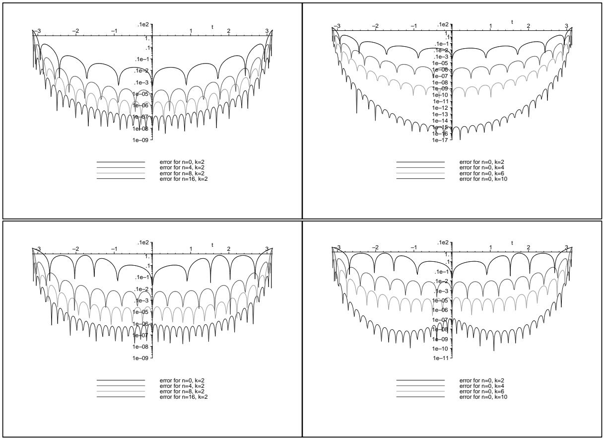
Figure 4: The modulus of the error of approximation on a logarithmic scale of the Fourier series of f_1(t) = s(t - \pi) (on the top) and of f(t) = f_1(t) + (1 - \cos(t))^3 s(t) (on the bottom). On the left we display the error for \epsilon_4^{(2\ell)} and on the right for \epsilon_{4+2\ell}^{(0)} , \ell = 0, 2, 4, 8 .
