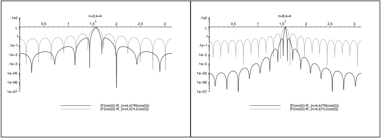
Figure 2: The modulus of the error of approximation on a logarithmic scale at x = \cos(t) of the linear and the nonlinear Padé-Chebyshev approximant of F(x) = \text{sign}(x) .
