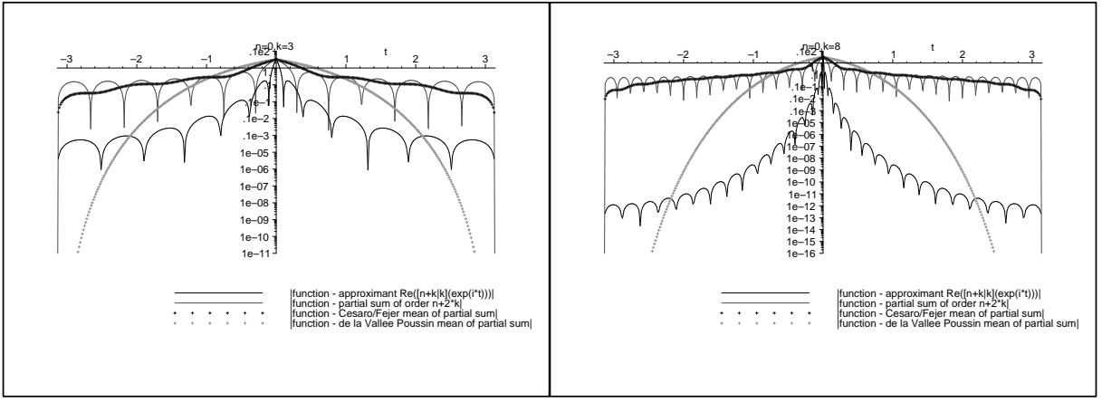
Figure 1: The modulus of the error of approximation on a logarithmic scale of the Fourier series of the saw tooth function (1.2). On the left we use the first 7 and on the right the first 17 coefficients of the Fourier series. The error for the partial sums is strongly oscillating, and, according to the Gibbs phenomenon, remains quite large (about 1/10) even for higher order Fourier sums. The error for Cesaro means is smoother, but about of the same size, even for arguments far from 0, the singularity of our function, whereas the de la Vallée-Poussin mean gives better approximants only far from 0. In contrast, the errors for \epsilon_6^{(0)} and \epsilon_{16}^{(0)} are much smaller, even for arguments closer to the singularity.
