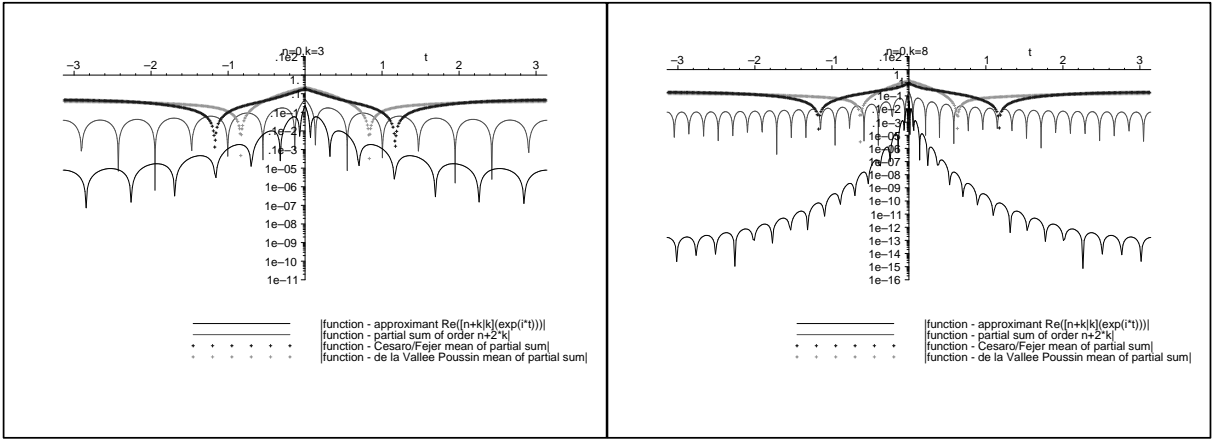
Figure 3: The modulus of the error of approximation on a logarithmic scale of the Fourier series of f(t) = |\sin(\frac{t}{2})| . On the left we use the first 7 and on the right the first 17 coefficients of the Fourier series.
